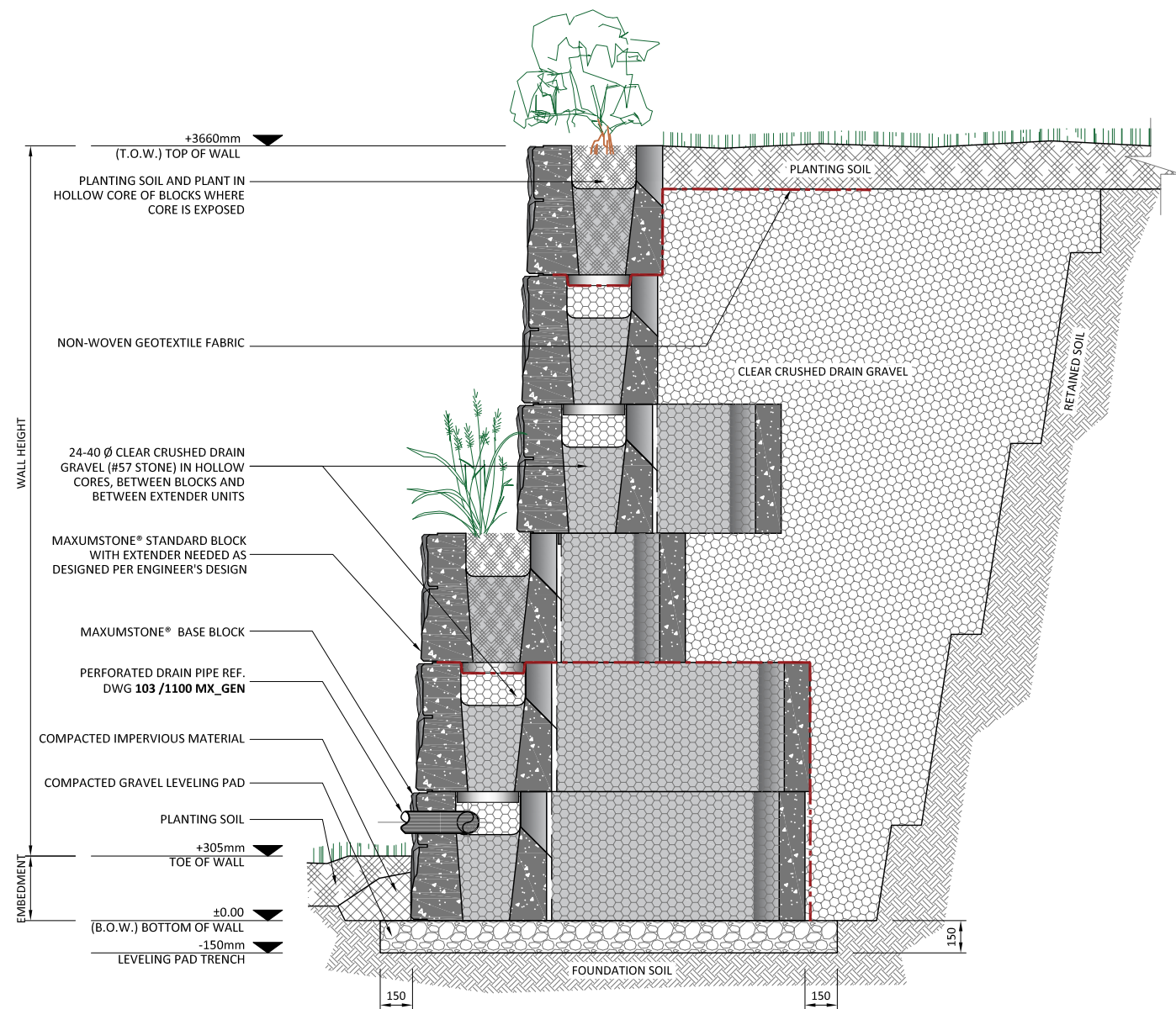
01 CROSS SECTION - OPTION 2 SCALE 1:30
