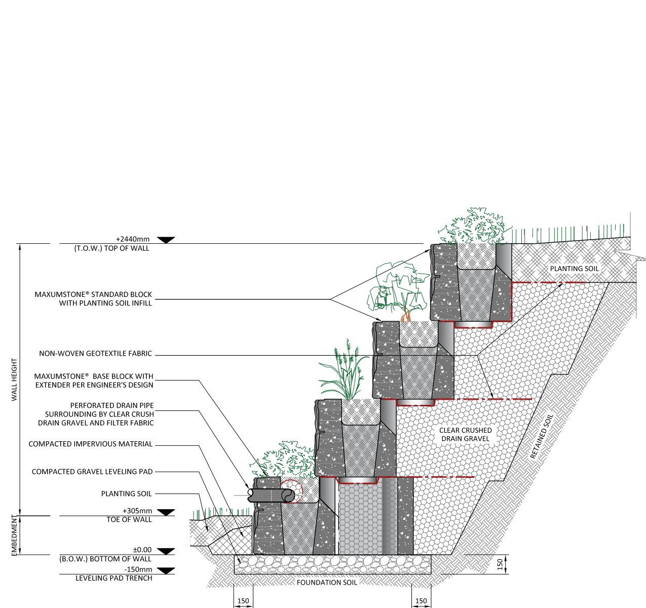
02 CROSS SECTION - OPTION 3 SCALE 1:30
